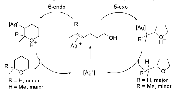
Scheme 1. Proposed Mechanism for Hydroalkoxylation
